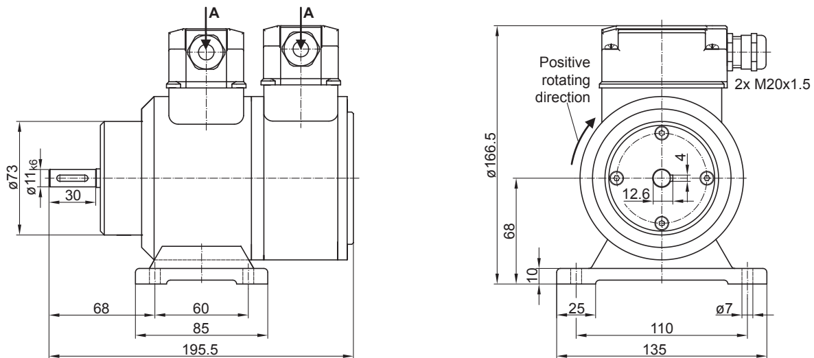
Housing foot B3
